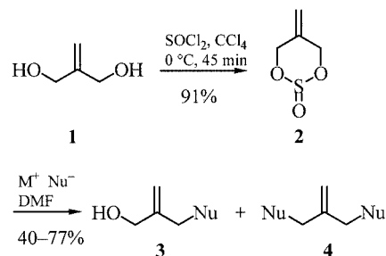
Scheme 1. Preparation of 5-methylene-2-oxo[1,3,2]dioxathiane ( 2 ) and its reaction with different nucleophiles; for details, see Table 1
