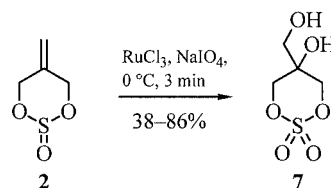
Scheme 3. Oxidation of 5-methylene-2-oxo[1,3,2]dioxathiane ( 2 ) to 5-(hydroxymethyl)-2,2-dioxo[1,3,2]dioxathian-5-ol ( 7 ); for details, see Table 2
