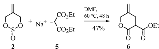
Scheme 2. Reaction of 5-methylene-2-oxo[1,3,2]dioxathiane ( 2 ) with diethyl sodiomalonate
